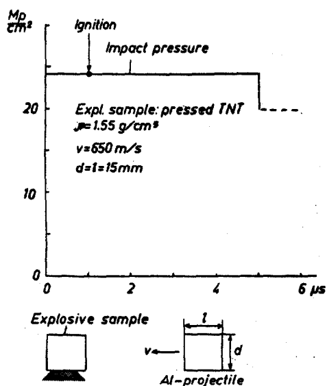
Fig 15 Shooting test
